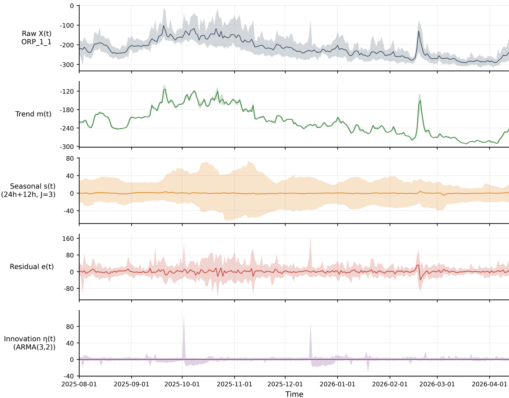
Full-span daily overview — ORP_1_1 (anaerobic, min) [2025-08-01~2026-04-13]
